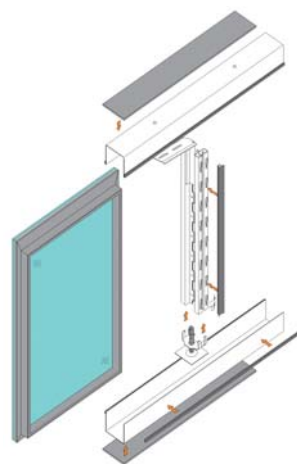
Lindner glass partition wall
