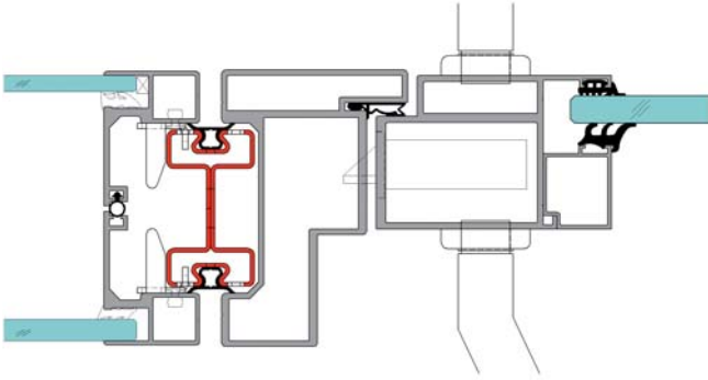
Aluminium architraves for the Campeon in Munich
